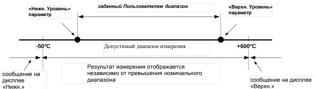
Fig. 6.1. Definition of measurement ranges
